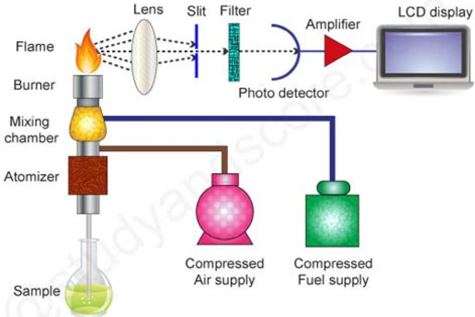
FLAME PHOTOMETER
