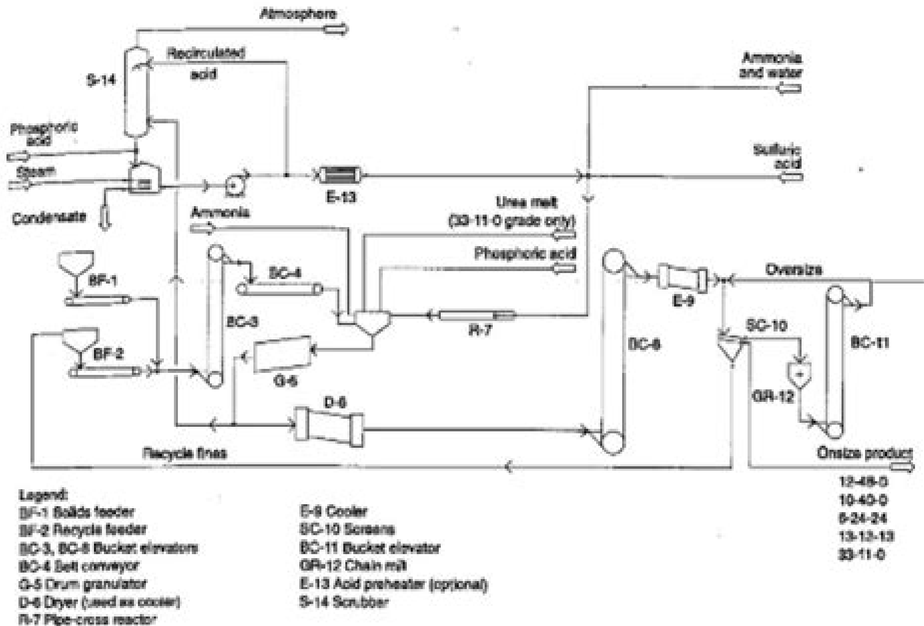
Figure 1. The TVA ammonium phosphate sulphate process
