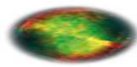
DUMBBELL NEBULA
