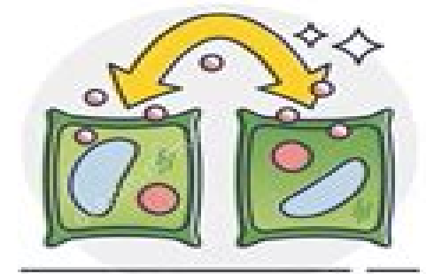
CELLULAR INTERACTIONS
